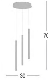
6139-3 15W LED-4000K
